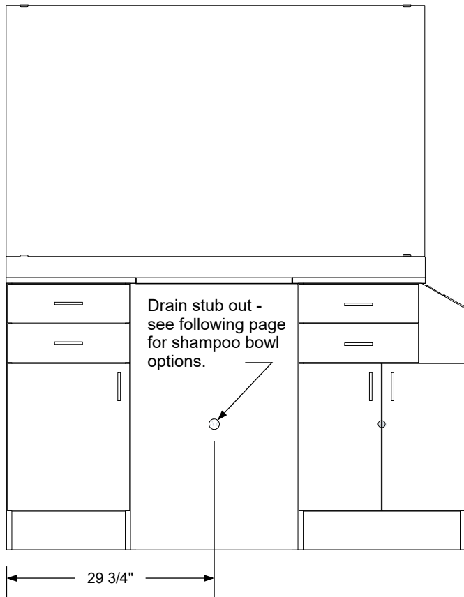
Plumbing stub out detail
