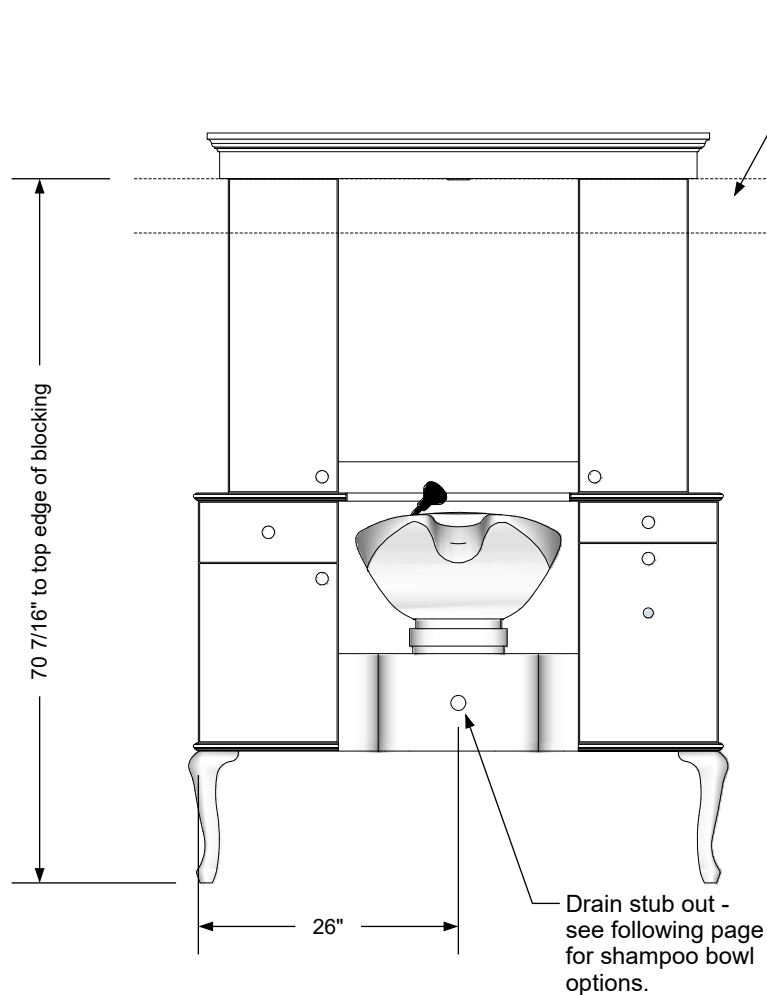
Plumbing stub & blocking detail
