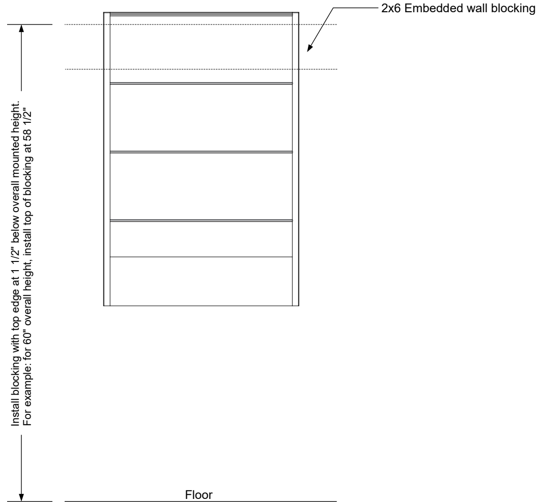
Wall blocking detail
