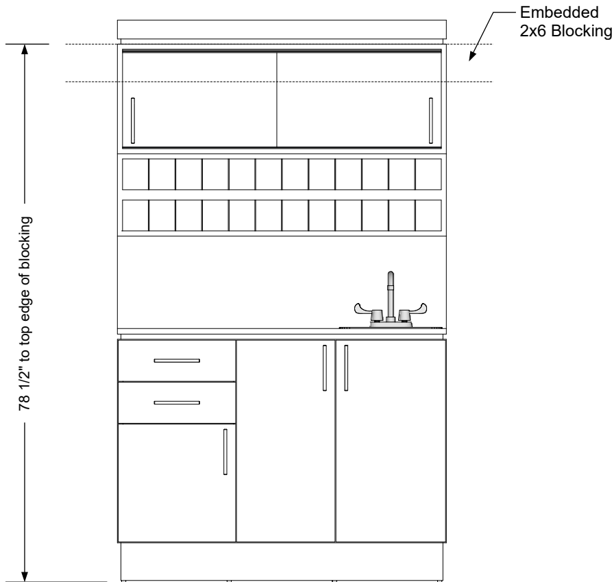
Blocking detail
