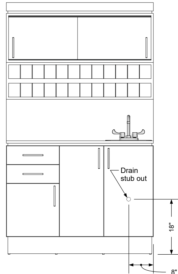
Plumbing stub out detail
