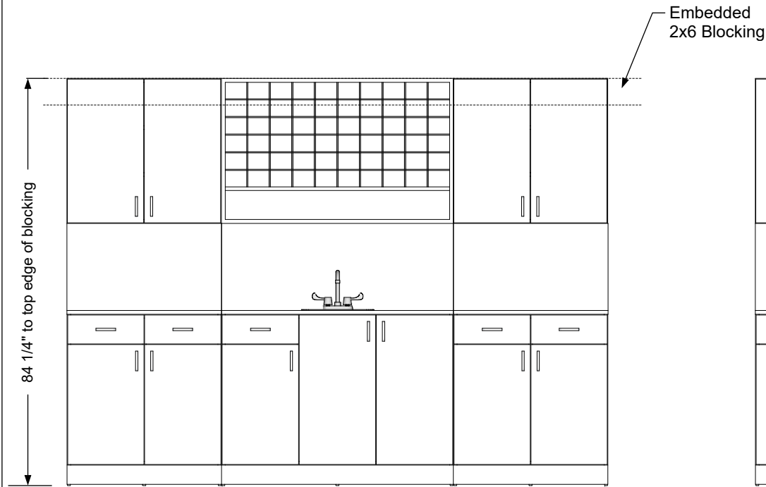
Blocking detail
