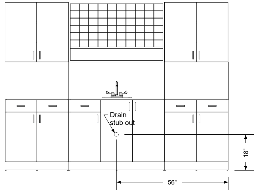
Plumbing stub out detail
