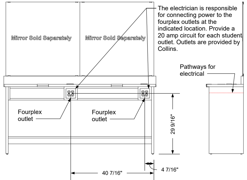
Electrical stub out detail
