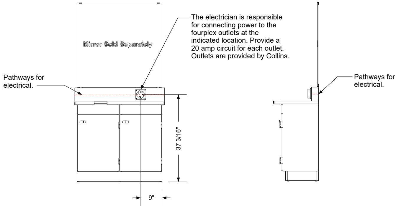
Electrical stub out detail
