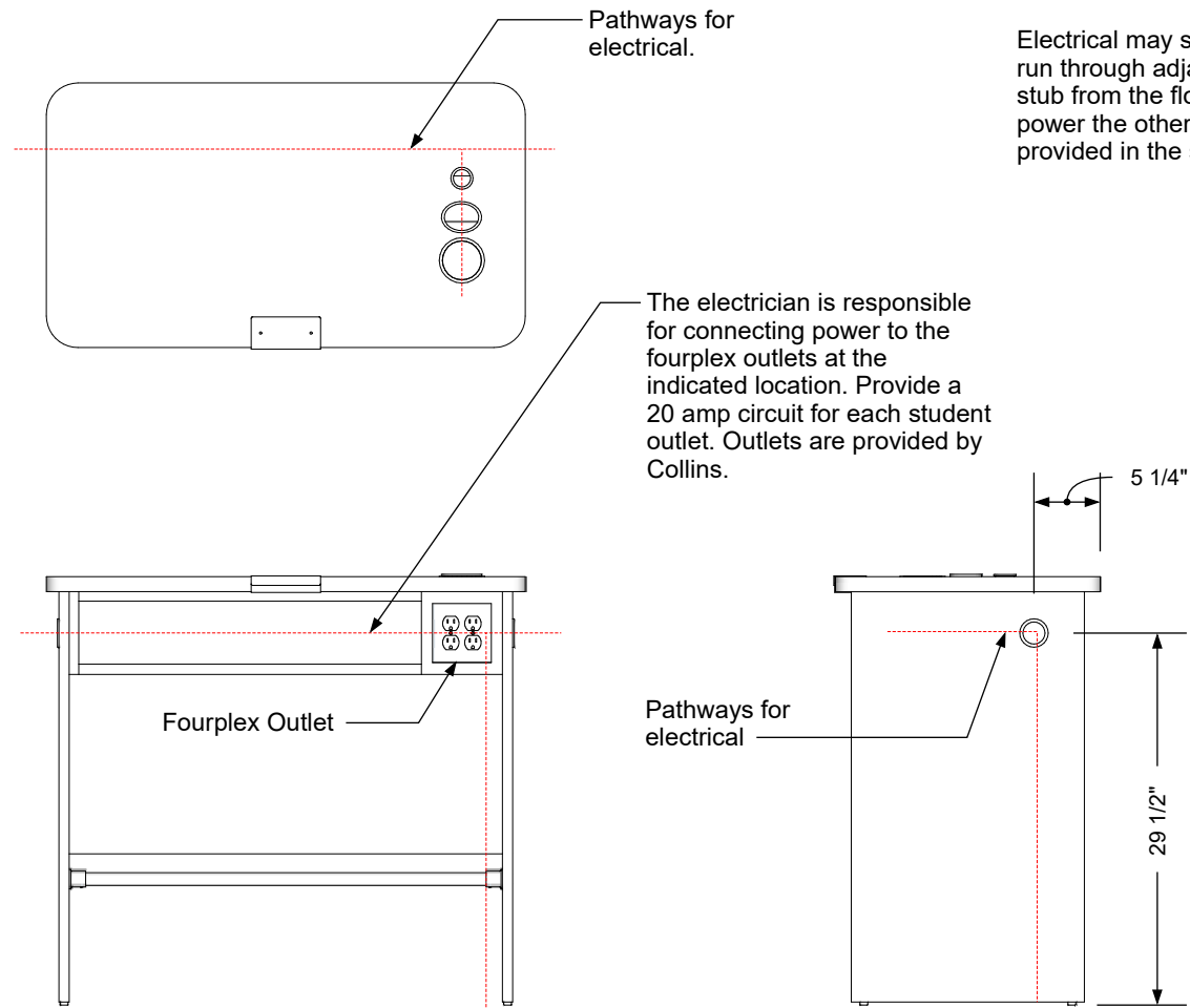
Electrical stub out detail
