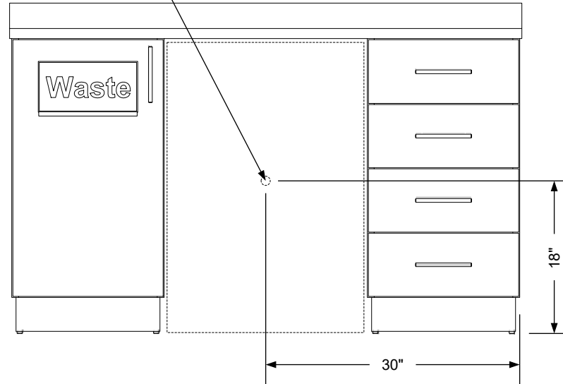
Electrical stub out detail
