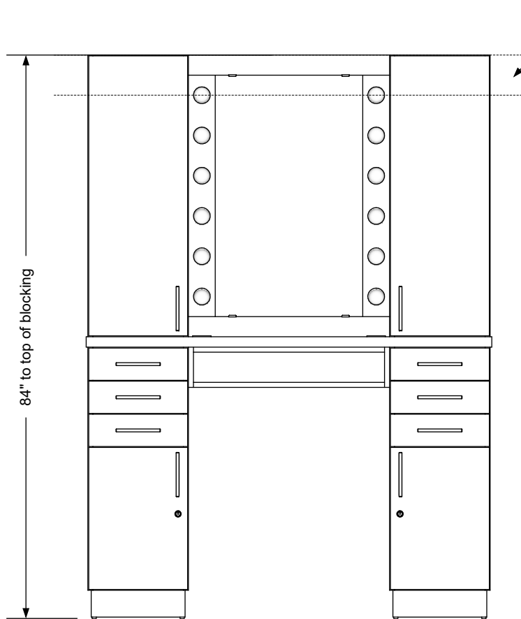
Wall blocking detail
