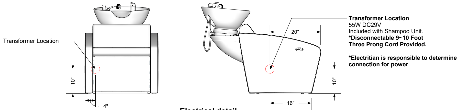
Electrical detail
