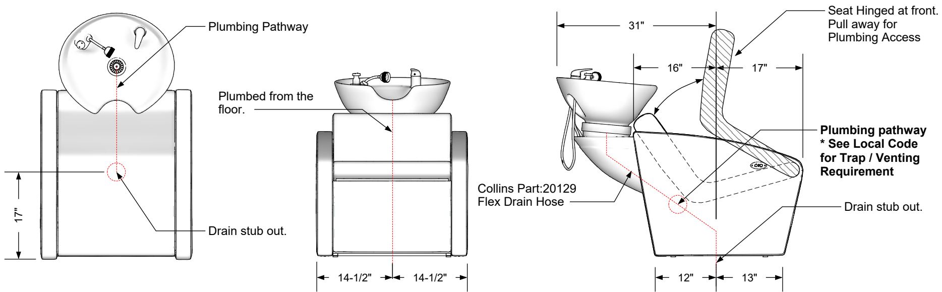
Plumbing stub out detail *Please Consult Local Codes
