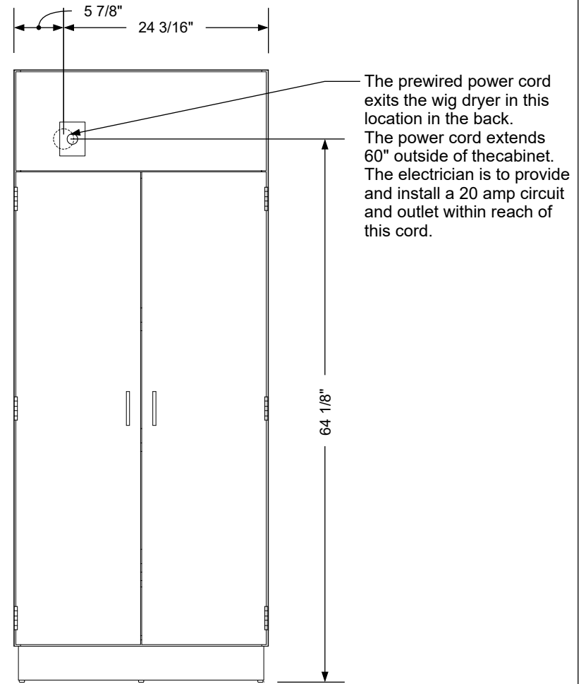
Electrical stub out detail
