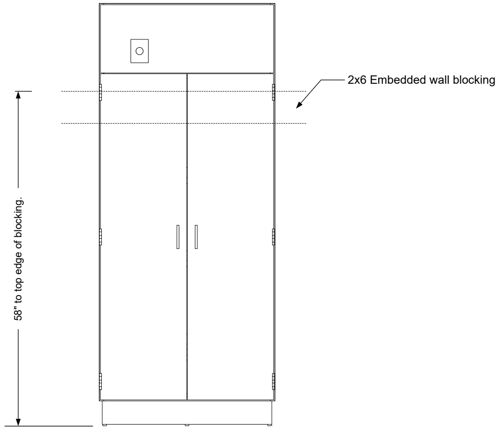
Wall blocking detail
