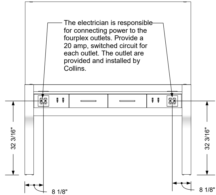
Electrical stub out detail
