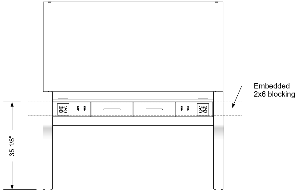
Wall blocking detail
