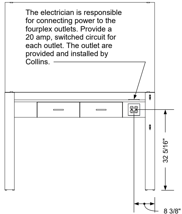
Electrical stub out detail
