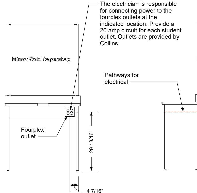
Electrical stub out detail
