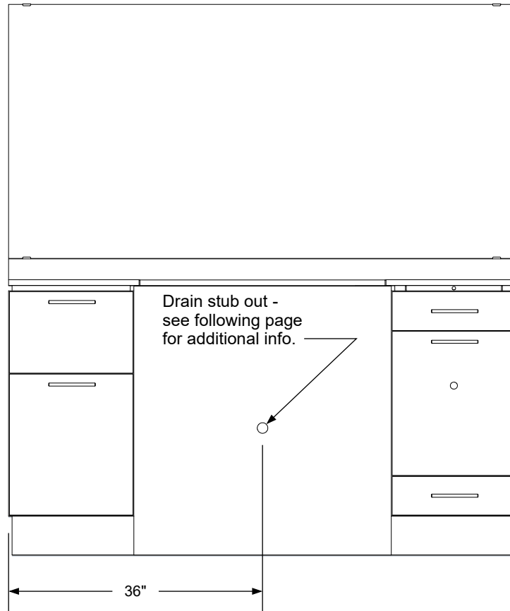
Plumbing stub out detail
