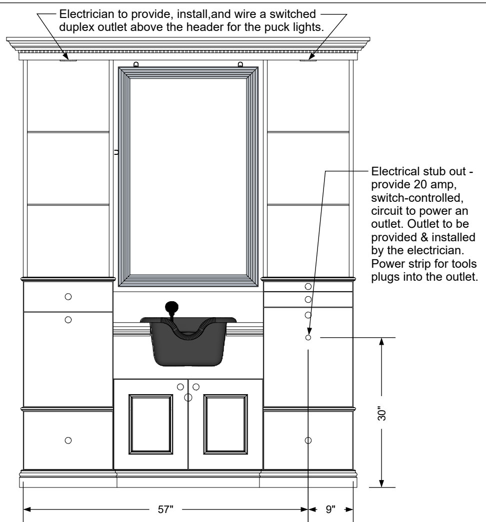
Electrical stub out detail
