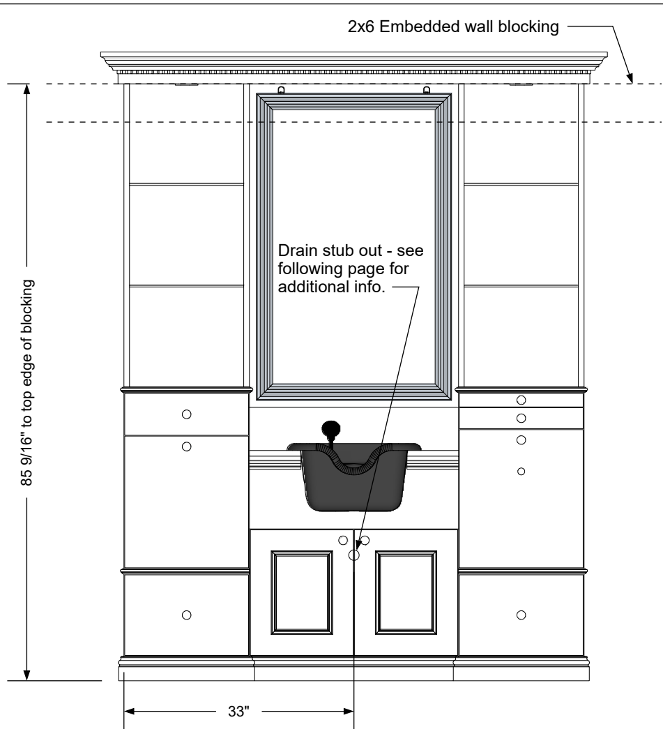
Plumbing stub & blocking detail
