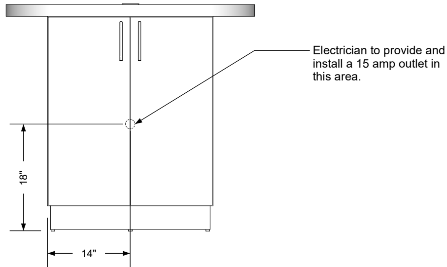
Electrical stub out detail
