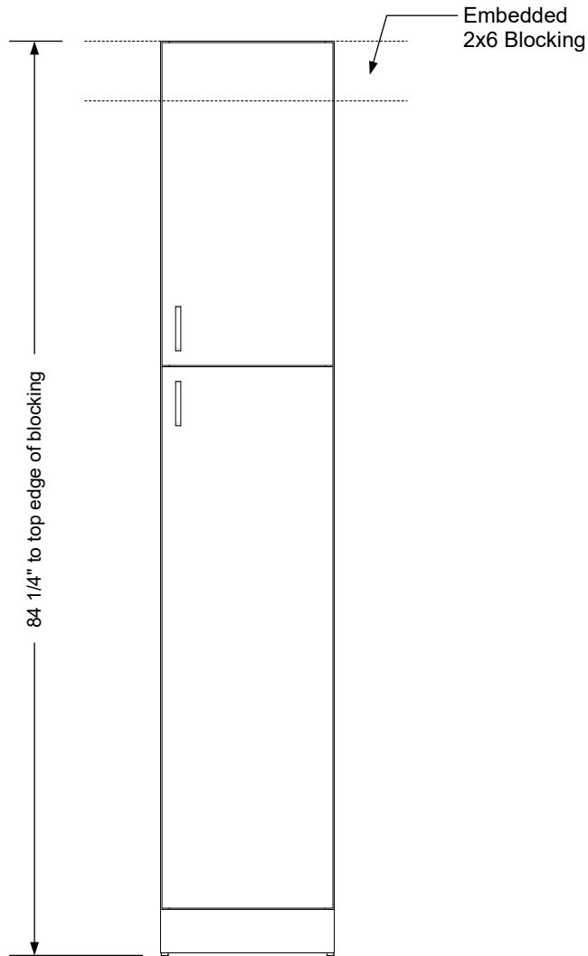
Blocking detail
