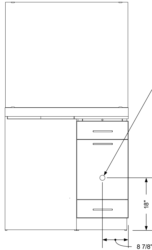
Electrical stub out detail
