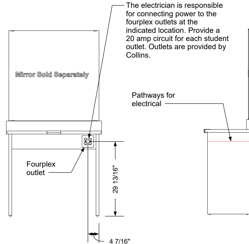
Electrical stub out detail
